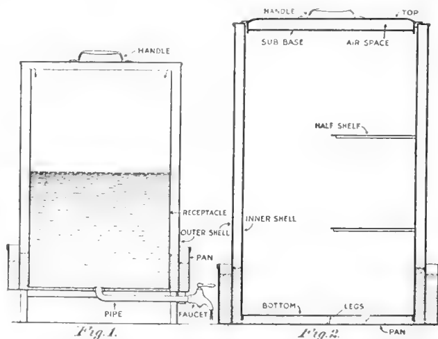
The Faucet Permits the Water to Be Drawn From the Shell Without Disturbing the Water in the Pan
